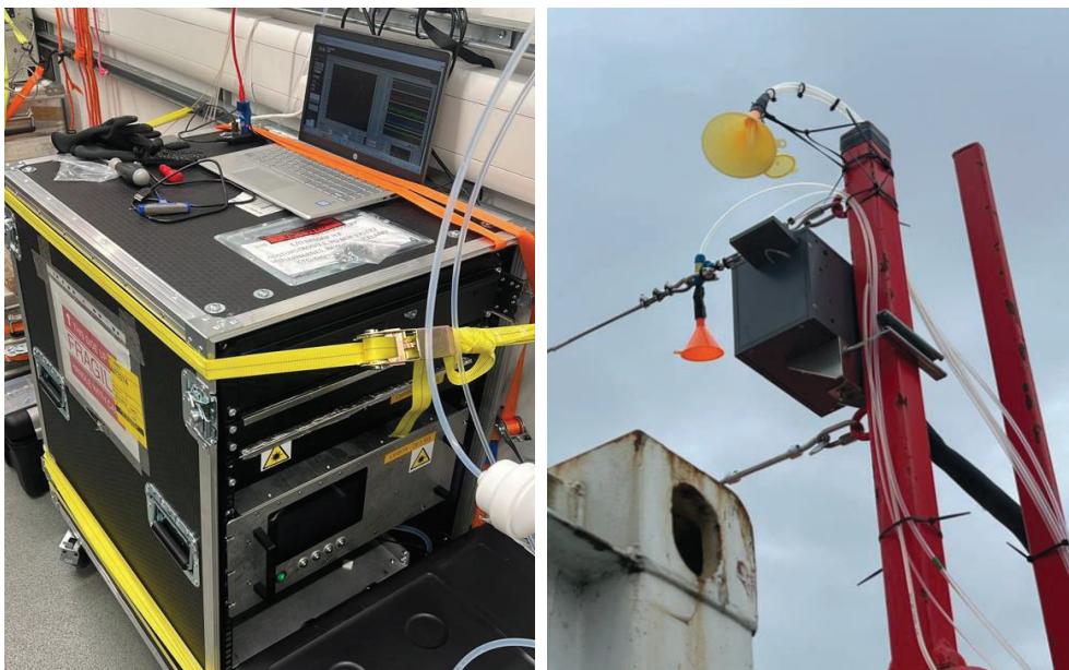
Figure 18. Photographs of the LIF-SO 2 instrument in the rack (left) and the SO 2 inlet on the roof of the BAS container (right), covered by an orange funnel (marked with an arrow).
