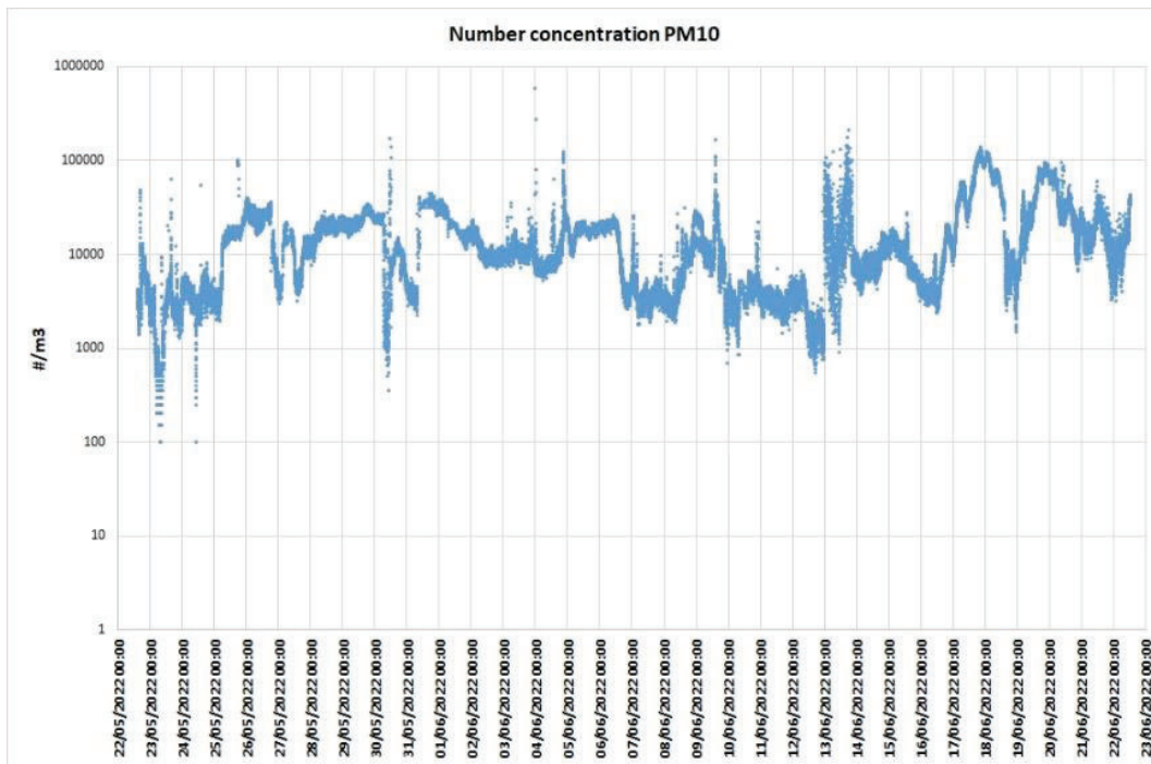
Figure 23: Number concentration per cubic metre of particles with a diameter between 0.25 and 10 \mu m (top). Mass concentration per cubic meter of particles with diameters between 0.25 and 10 \mu m (bottom).
