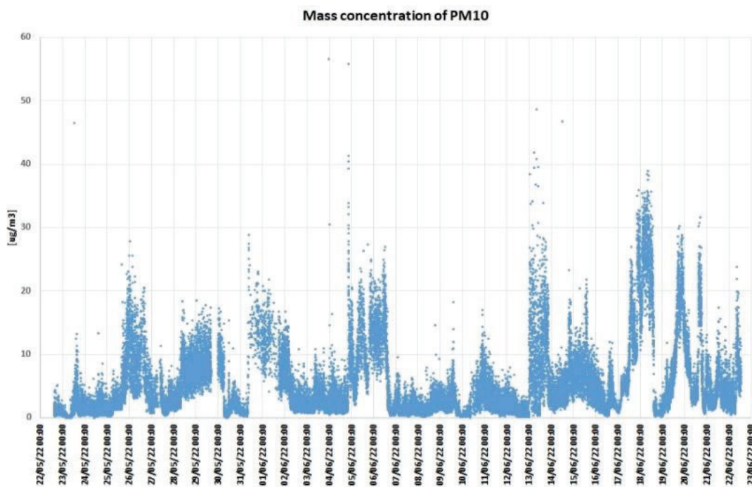
Figure 24: Mass concentration per cubic meter of particles with diameters between 0.25 and 10 \mu m.
