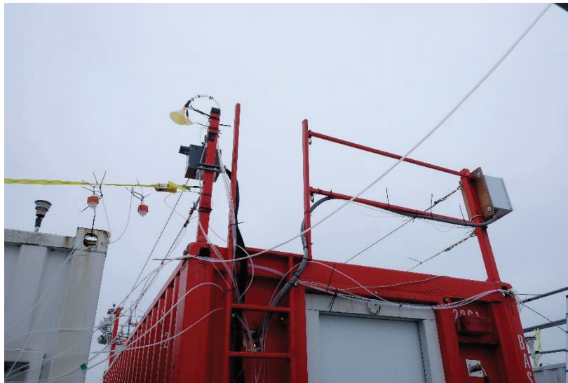
Figure 14. Photograph of the O 3 , NO x , SO 2 and CO inlets on the left (covered by the big and small funnel) and the NO y converter box on the right of the roof of the BAS container.
